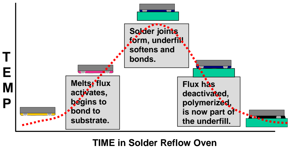
Figure 6 – Reflow Profile
