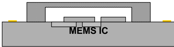
Figure 8 – Cap-on-Chip
