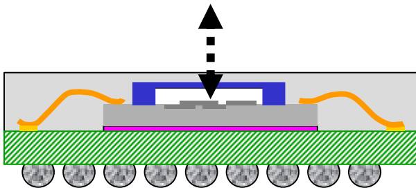
Figure 9 – Optical MEMS package
