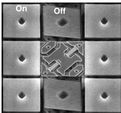
Figure 6 - DMD™ Structure [3]
