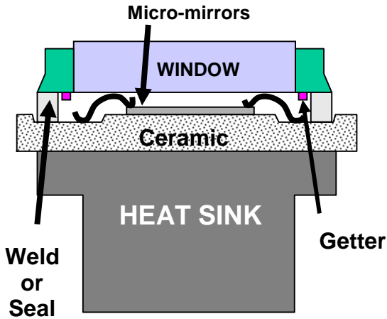
Figure 5 – MOEMS Package Design
