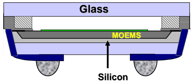
Figure 7 - ShellOp
