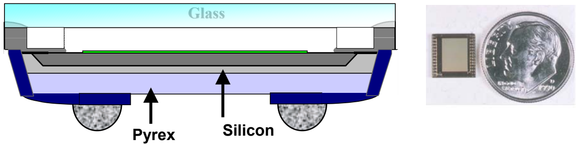
Figure 7 – ShellOp (ShellCase)
